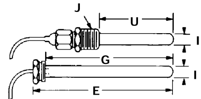
GAS SERVICE BULB & WELL DIMENSIONS inches (mm)
