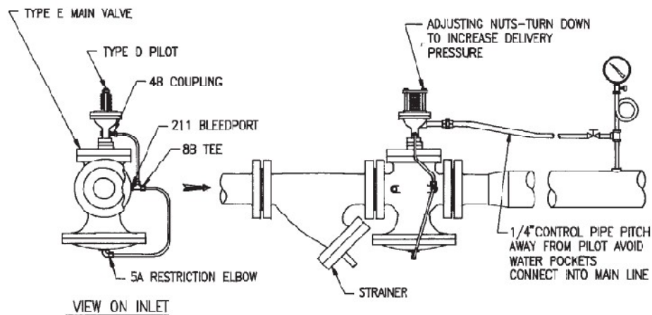
FIGURE 1B - Installation of Integrally Mounted Pilot
