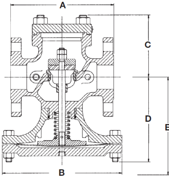
TYPE E MAIN VALVE
