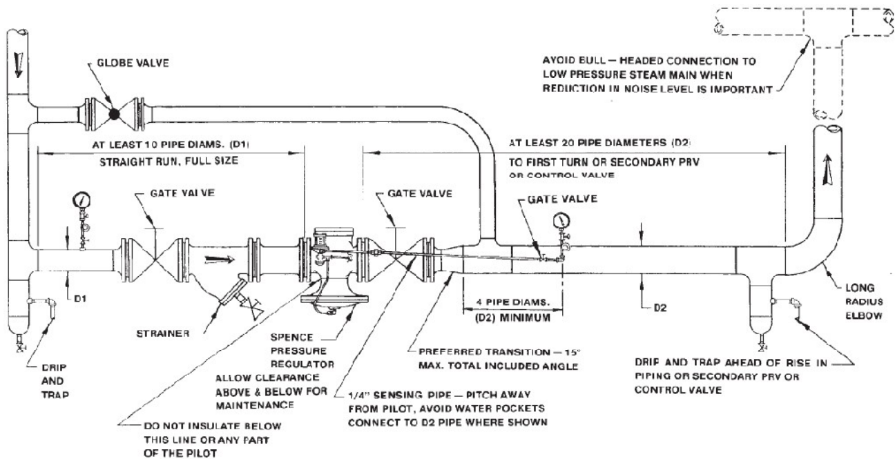
FIGURE 1A - Typical Installation
