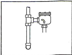
Fig. 4.4 – Dirt pocket made from pipe fittings when a strainer is not available. Clean dirt pockets and strainers frequently.
