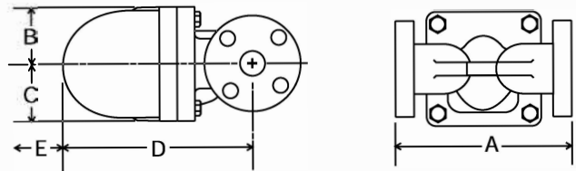
FTE-43 CAST IRON 1/2" &amp; 3/4"
