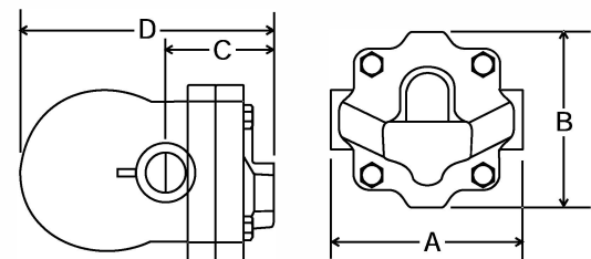
FTE-14-DUCTILE IRON 1/2", 3/4" & 1"
