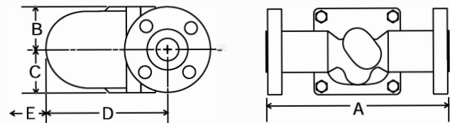
FTE-44F CAST STEEL 1/2" &amp; 3/4"
